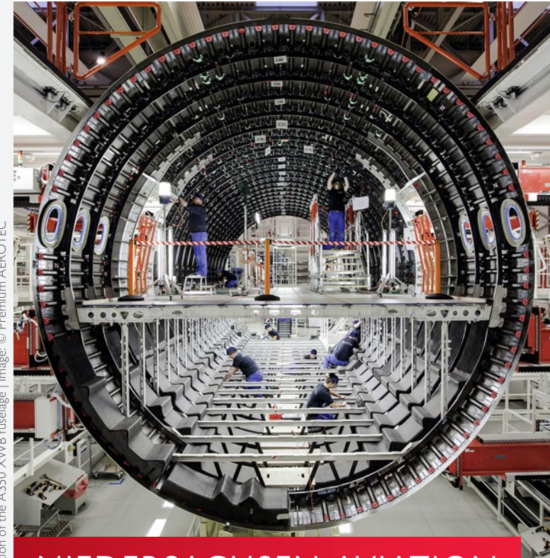
Production of the A350 XWB fuselage | Image: © Premium AEROTEC
